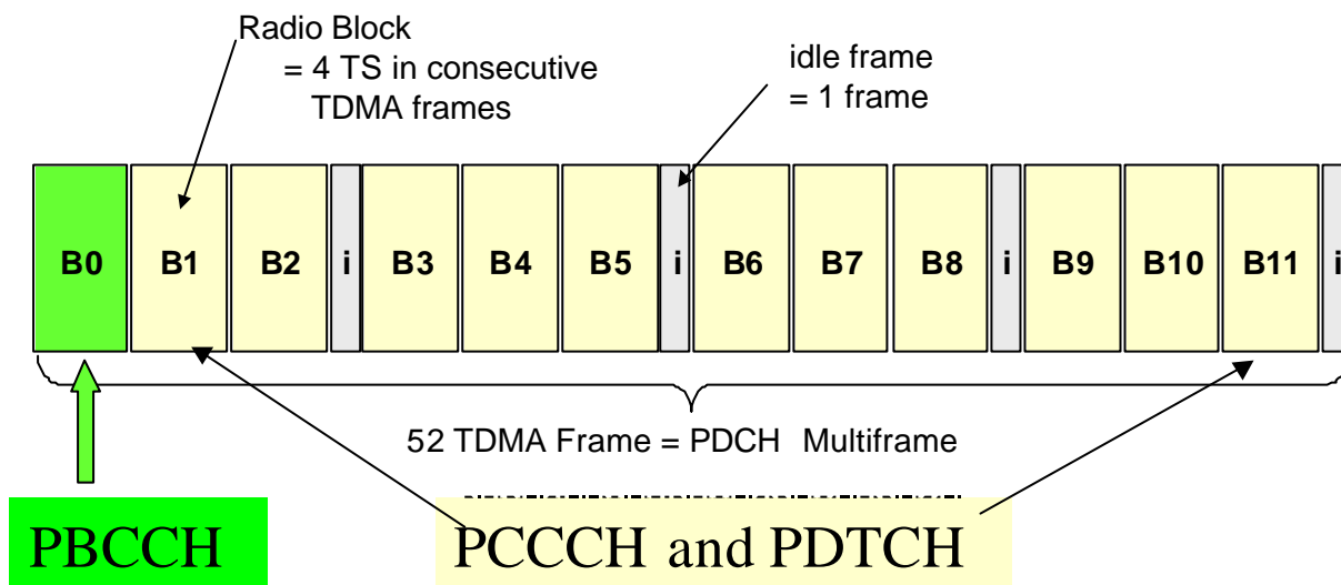
Figure: Position of the PBCCH within a 52-multiframe
